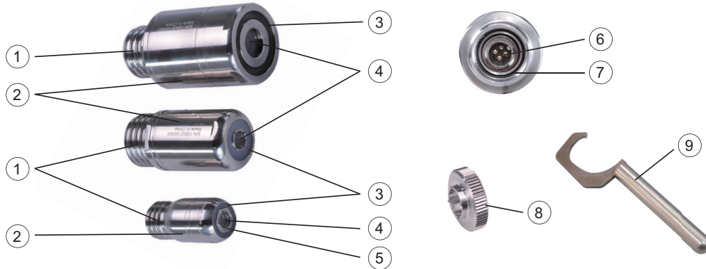
Cameras for the Type-CP and Type-M2 Reels
